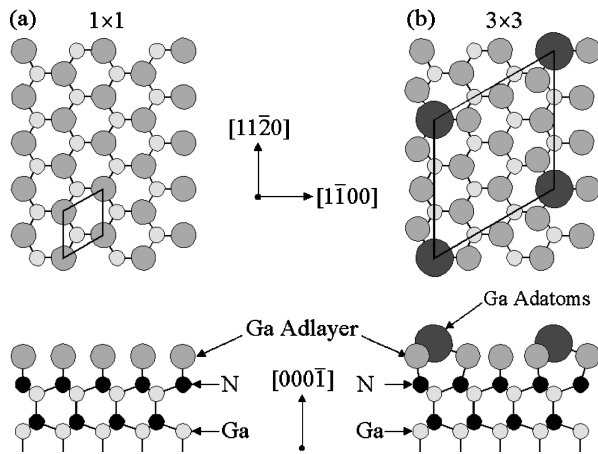
FIG. 1. Model structures determined for the (a) 1\times 1 Ga adlayer structure and (b) 3\times 3 adatom-on-adlayer structure of GaN(000 \bar{1} ). The Ga adlayer is under tensile stress since the Ga atoms are stretched further apart compared to their spacing in bulk Ga (3.19 Å compared \sim 2.7 Å). For the 3\times 3 structure, the adlayer atoms are able to get closer together by moving in the in-plane (lateral) direction away from the Ga adatoms by 0.51 Å, thus relieving the stress. All other lateral or vertical displacements of the adlayer atoms are less than 0.1 Å.
