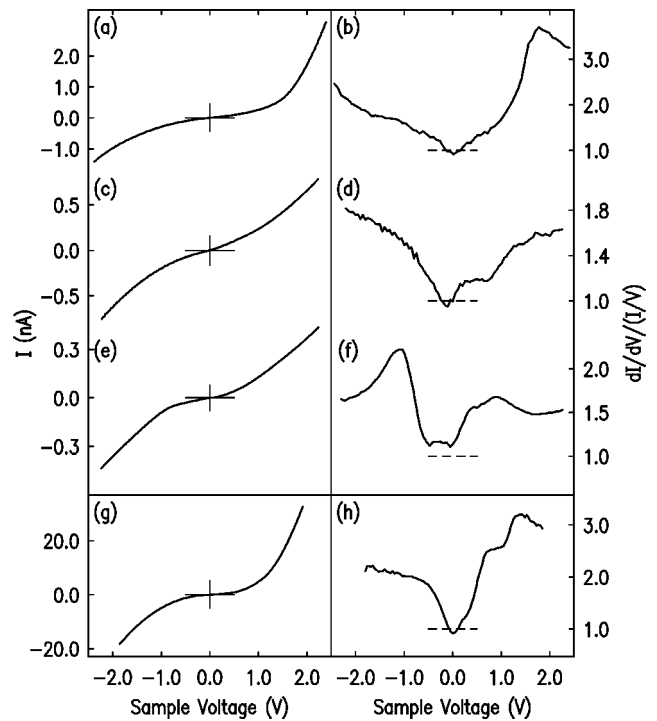
FIG. 3. Averaged tunneling spectroscopy results from three separate experiments (three different tips) on the GaN(000 \bar{1} )1 \times 1 surface (a)-(f) and a single experiment on the GaN(0001) "1 \times 1" surface (g) and (h). I - V curves are shown on the left with the corresponding normalized conductance curves shown on the right. Crossmarks represent the origins for the I - V curves, while dashed lines indicate where the normalized conductance=1.
