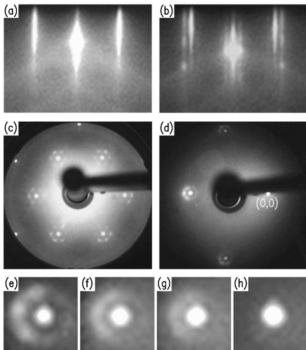
Fig. 4. 1 \times 1 RHEED pattern for GaN(0001) (a) during growth, and (b) after cooling to below 350^\circ\text{C} , where it converts to a 1 + \frac{1}{6} pattern. The 1 + \frac{1}{6} LEED pattern ( E_{\text{inc}} = 100 \text{ eV} ) is shown in (c). For most “ 1 \times 1 ” surfaces (see the text), a 1 + \frac{1}{12} pattern is observed below 200^\circ\text{C} , as shown in (d) ( E_{\text{inc}} = 40 \text{ eV} ). LEED in the vicinity of the (0, 1) spot ( E_{\text{inc}} = 40 \text{ eV} ) at various temperatures: (e) room temperature– 100^\circ\text{C} , (f) 100 – 150^\circ\text{C} , (g) 150 – 200^\circ\text{C} , and (h) above 350^\circ\text{C} .
