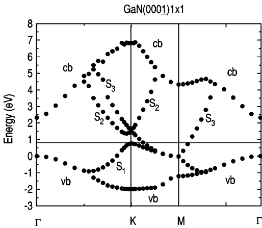
FIG. 2. Band structure for the GaN(000 \bar{1} )1 \times 1 Ga adlayer based on local density functional calculations. Energies are plotted relative to the VBM. The Fermi level is located 0.75 eV above the VBM. The plot shows the valence and conduction band edges and three surface states: S_1 , S_2 , and S_3 . The computed bulk band gap of GaN is less than the experimental value (3.4 eV).
