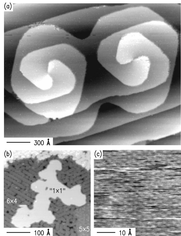
Fig. 5. STM images of (a) GaN(0001) “ 1 \times 1 ” surface showing spiral growth, (b) (0001) surface with mixed 5 \times 5 , 6 \times 4 , and “ 1 \times 1 ” reconstructions (“ 1 \times 1 ” island height = 2.1 \text{ \AA} ), and (c) “ 1 \times 1 ” reconstruction showing atomic resolution [lateral spacing = GaN lattice constant ( 3.19 \text{ \AA} ) to within < 1\% ]. The tunnel parameters are (a) -2.0 \text{ V} at 0.1 \text{ nA} , (b) -2.5 \text{ V} at 0.075 \text{ nA} , and (c) -0.25 \text{ V} at 0.1 \text{ nA} . The atomic steps seen in (a) are single bilayer high ( 2.59 \text{ \AA} ) (line-by-line background subtraction has been applied to permit viewing of many terraces). The gray scale ranges are (b) 4.0 and (c) 0.27 \text{ \AA} , respectively.
