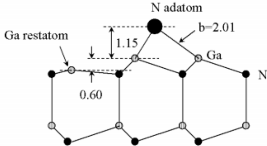
N-adatom in H3 site on GaN(0001)
