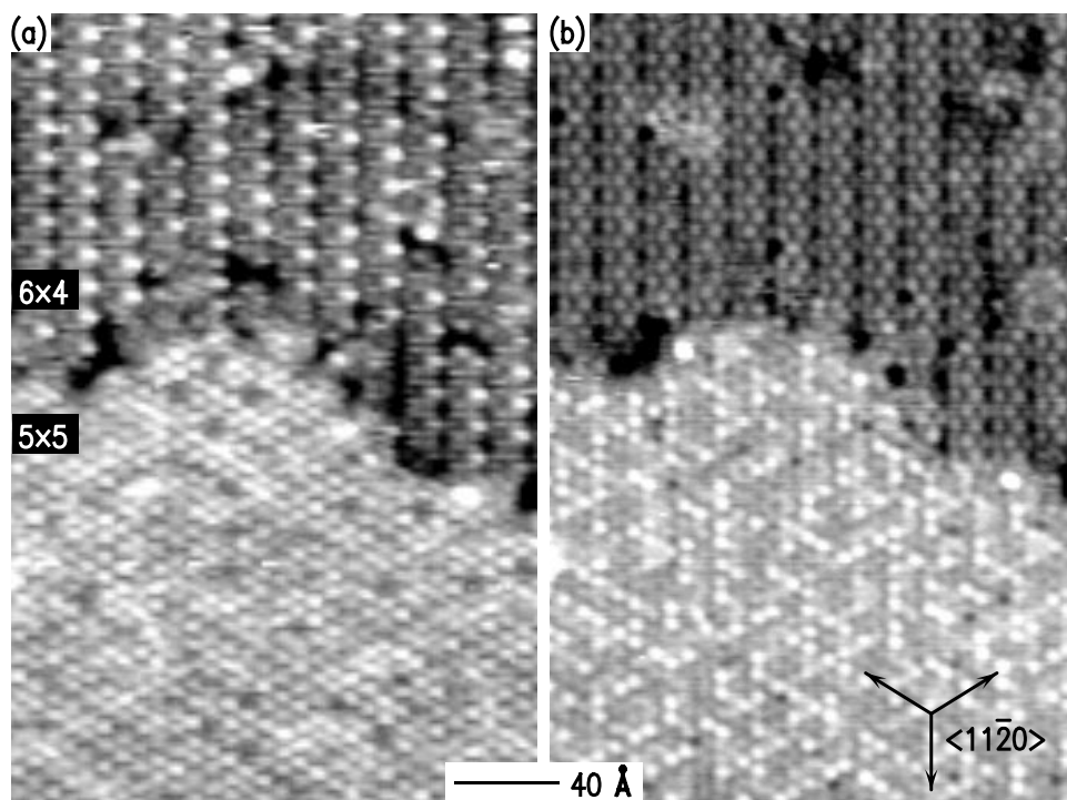
Figure 6 Dual bias images of the 5 \times 5 and 6 \times 4 reconstructions. The average height difference between the two reconstructions is 0.3 Å for empty states (+1.0 V sample voltage) shown in (a) and 0.4 Å for filled states (-1.0 V sample voltage) shown in (b), with the 5 \times 5 being higher in each case. In both images the total gray scale range is about 1.3 Å.
