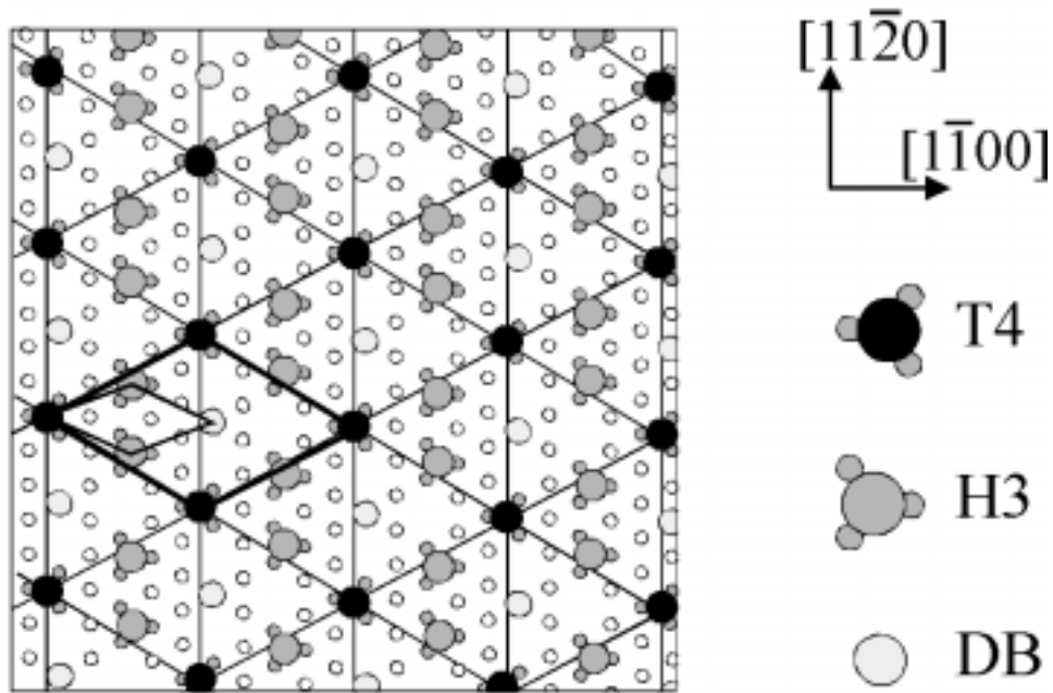
Figure 13 Structural model for the 5 \times 5 reconstruction. Ga-adatoms in T4 sites and N-adatoms in H3 sites are shown by large black and large grey circles respectively. The small open circles in the diagram represent the Ga rest atoms in the 2nd layer. In the locations where the small open circles are missing, Ga vacancies occur. The N atoms in the 3rd layer are not shown. The light grey circle labelled DB (dangling bond) is a particular Ga rest atom site. In an alternative model, this site could conceivably contain another adatom in a nearby T4 or H3 site.
