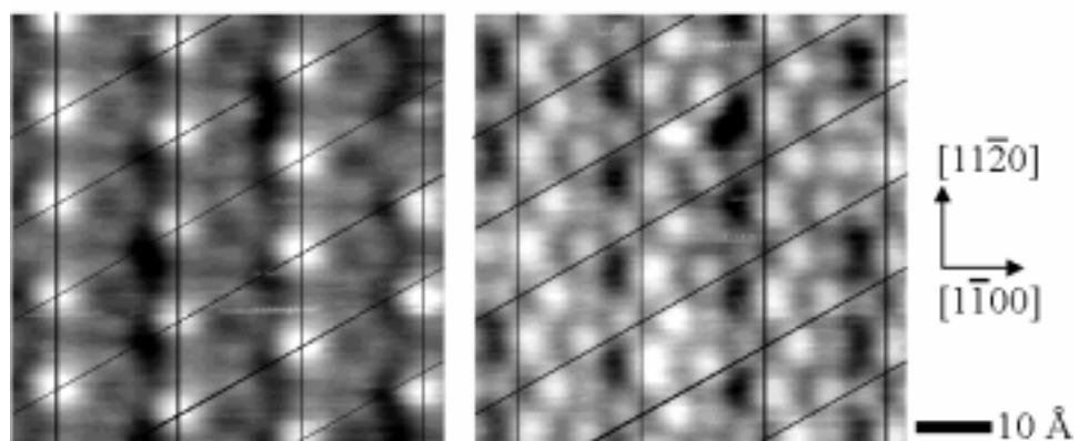
Figure 8 Simultaneously-acquired dual bias images of the 6\times 4 reconstruction overlaid with 6\times 4 grids. Sample biases and gray scale ranges are +1.0 V and 1.2 Å for (a) and -1.0 V and 0.8 Å for (b).
