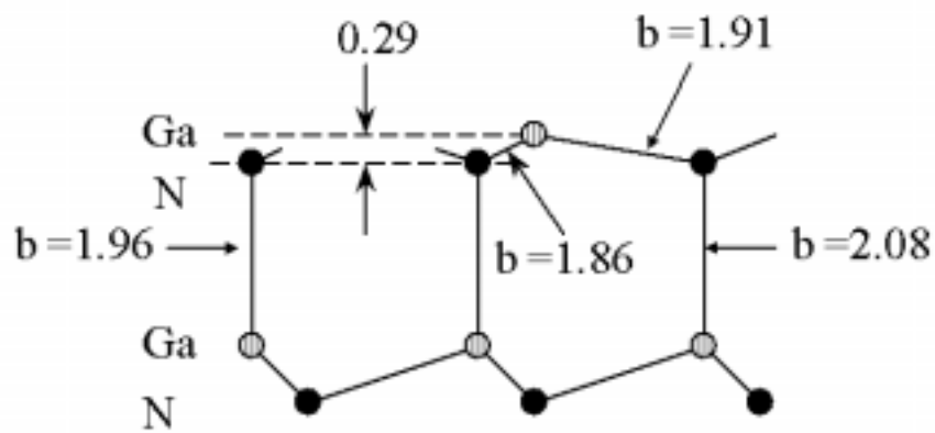
( 2 \times 2 ) Ga vacancy on GaN(0001)
