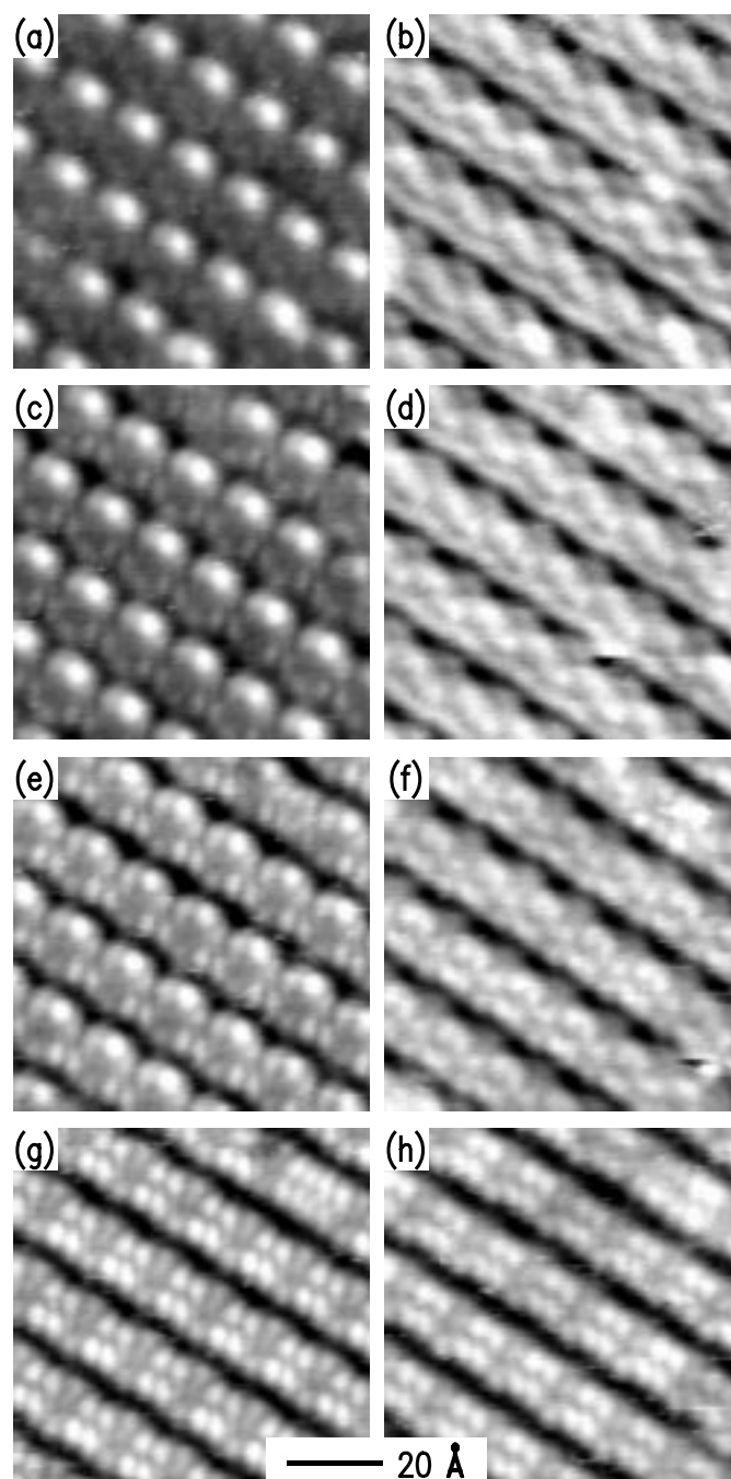
Figure 7 Simultaneously-acquired dual bias images of the 6\times 4 reconstruction. Sample biases are +2.0 and -2.0 V for (a) and (b), +1.5 and -1.5 V for (c) and (d), +1.0 and -1.0 V for (e) and (f), and +0.5 and -0.5 V for (g) and (h), respectively. Similarly, gray scale ranges are 1.1 Å and .7 Å for (a) and (b), 1.1 Å and 0.8 Å for (c) and (d), 1.1 Å and 0.9 Å for (e) and (f), and 1.3 Å and 1.3 Å for (g) and (h).
