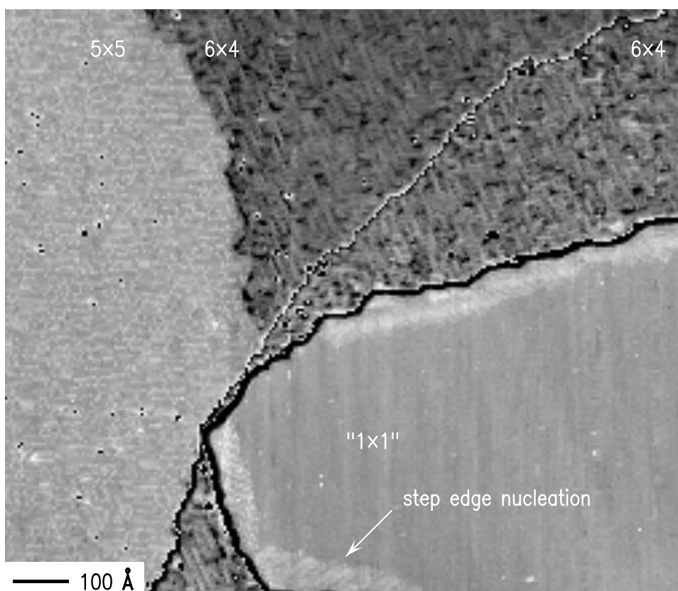
Figure 9 STM image of Ga-face showing 5\times 5 , 6\times 4 , and “ 1\times 1 ” reconstructions on three different terraces. The image is displayed with split gray scales to bring out the contrast on each terrace. The lowest terrace has both 5\times 5 and 6\times 4 domains. A single bilayer step running approximately from
