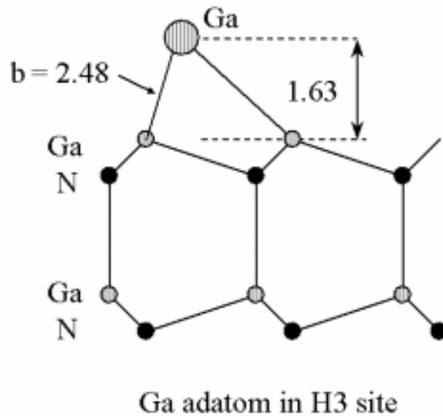
Figure 15 Schematic model of gallium H3 adatom structure. All dimensions are given in Å.
