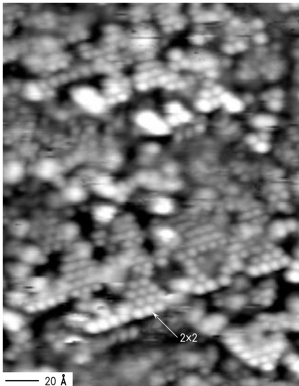
Figure 3 STM image of nitrided surface showing small ordered areas of 2x2 reconstruction. Sample bias = -2.0 V; tunnel current = 0.075 nA; gray scale range = 3.0 Å.
